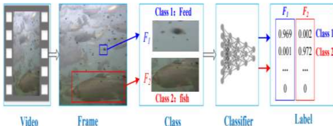
Figure 4. Species classification
